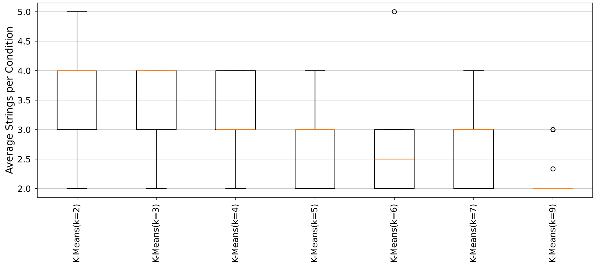
YARA Rules Average Strings per Condition Distribution (Cluster15_Size9 dataset)
